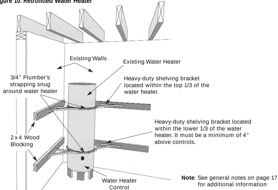
Figure 10: Retrofitted Water Heater
